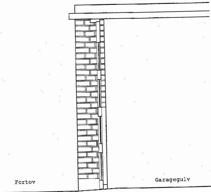
Snit i garageport 1:20
